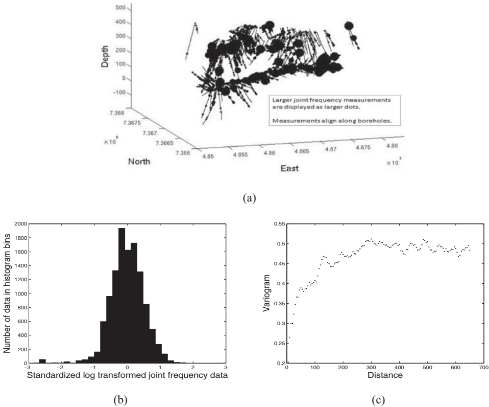
Figure 4. Mining data: (a) Data sites in a Norwegian iron mine. The data size is n = 11,107 , collected in about 200 boreholes. (b) Histogram of shifted log-transformed data of joint frequencies. (c) Empirical variogram.
