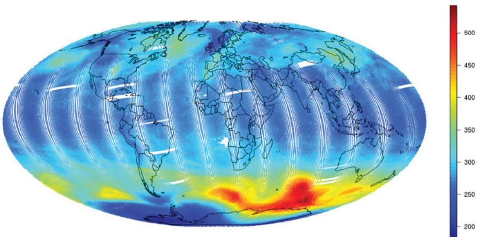
Figure 5. Total column ozone data: number of measurements is n = 173,405 .
