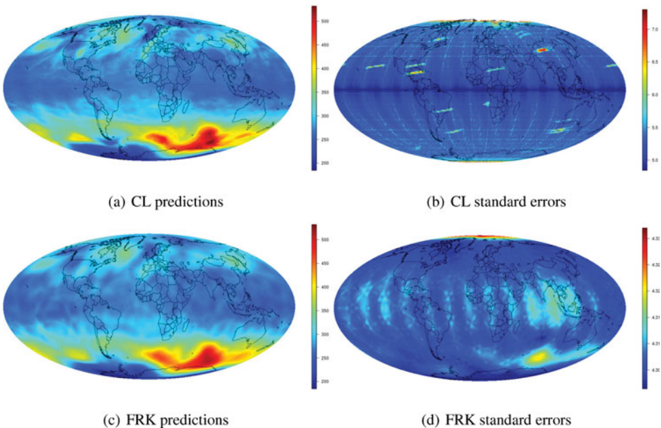
Figure 6. Total column ozone data: top displays are based on the CL model with 30 \times 30 longitude and latitude blocks. Bottom displays are based on fixed-rank kriging. Predictions ((a) and (c)) and prediction standard deviations ((b) and (d)).
