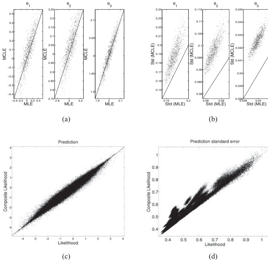
Figure 2. Synthetic data: comparison of full likelihood (x-axis) and CL (y-axis). (a) Estimates. (b) Asymptotic standard deviation of estimators. (c) Predictions. (d) Prediction standard deviations. The CL is based on 100 blocks. The number of prediction sites is 500, and results are computed over 1000 replicates of data at n = 2000 observation sites. \theta_1 is a precision parameter, \theta_2 is a range parameter, and \theta_3 is a nugget precision parameter.
