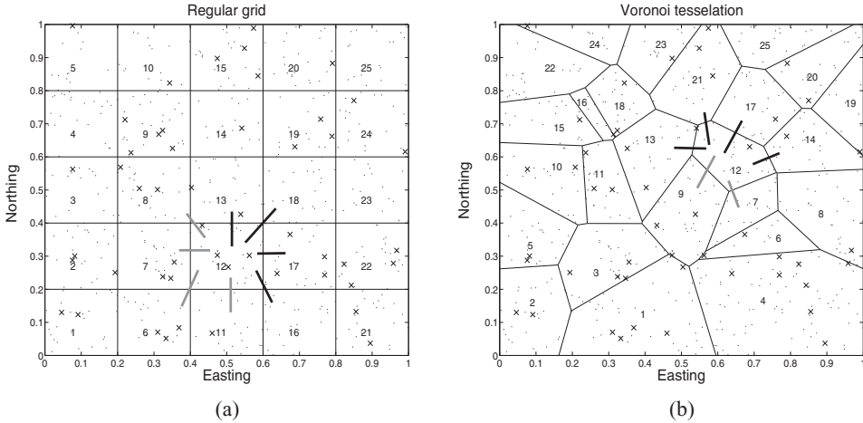
Figure 1. Observation sites illustrated by “x” and predictions sites by “x.” A block CL splits the spatial domain into regular (a) or irregular (b) blocks. Each block communicates pairwise with each of its neighbors. For the regular grid (a), an interior block has eight neighbors. For a random or adaptive grid (b), the number of neighbors varies. In both displays, the block indexed 12 has four neighbors with higher indices (black edges).
